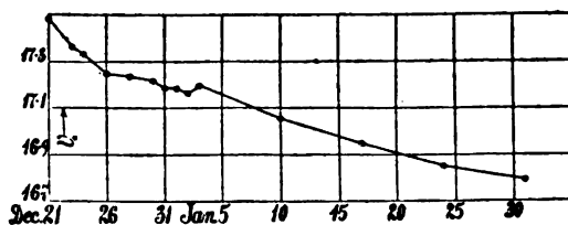
FIG. 25.—Chart showing loss of standard volumes of gas in diver in lapse of days. Diffusion of air through KCl solution.
